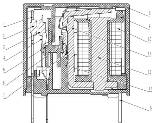
结构图Construction Schematic
